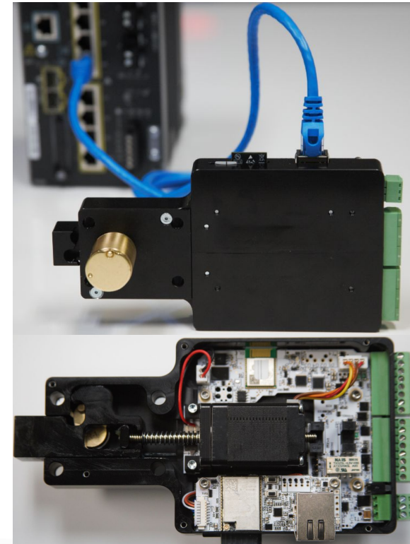
Electronic Smartlock
